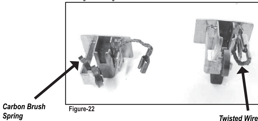
Removing and Installing the Carbon Brush
